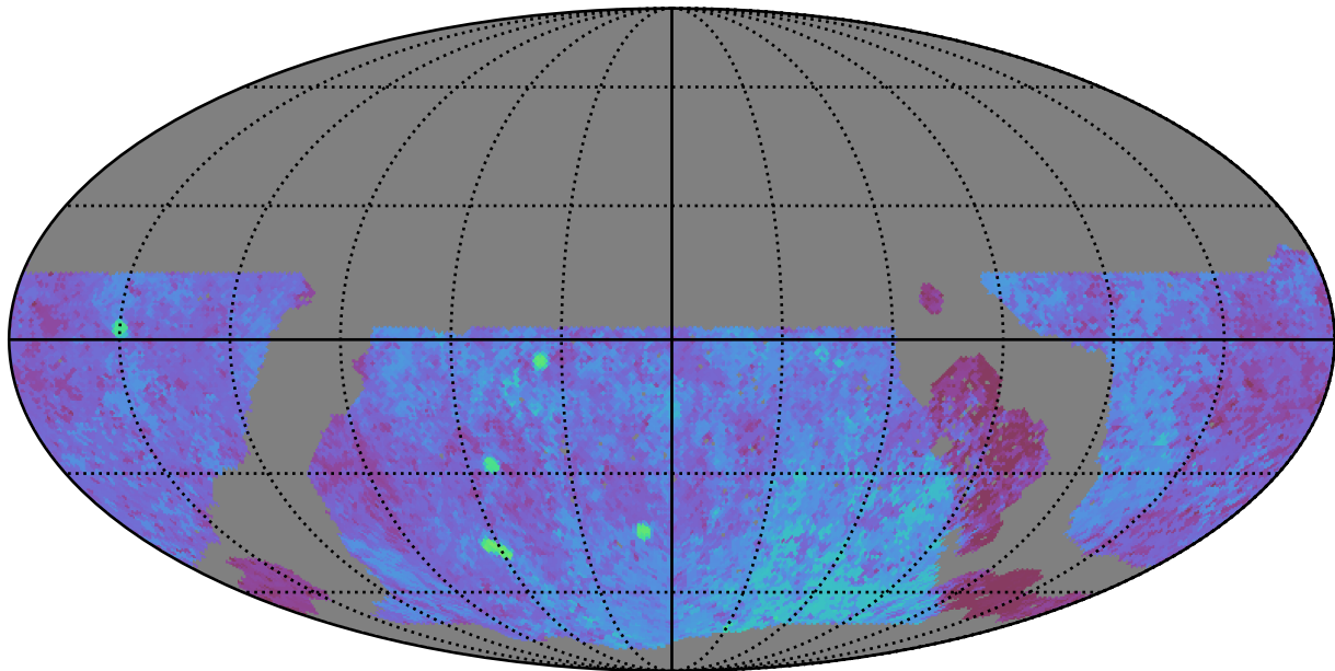
noroll_mjdp365_v3.4_10yrs WFD u band: Median Season Length
