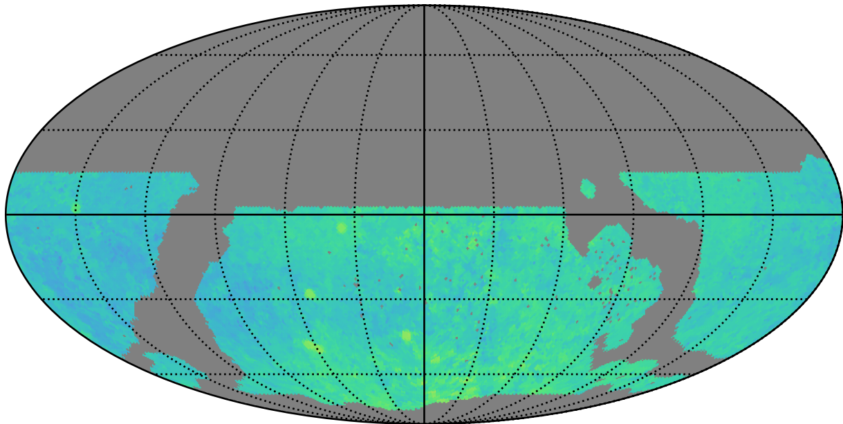
noroll_mjdp365_v3.4_10yrs WFD i band: Median Season Length
