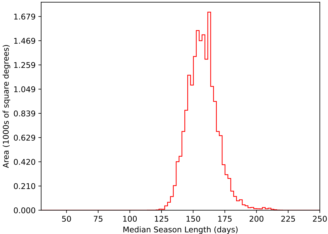
noroll_mjdp365_v3.4_10yrs WFD i band: Median Season Length
