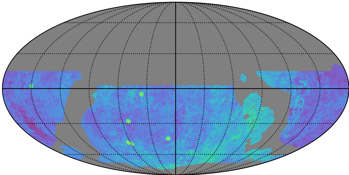
noroll_mjdp365_v3.4_10yrs WFD g band: Median Season Length
