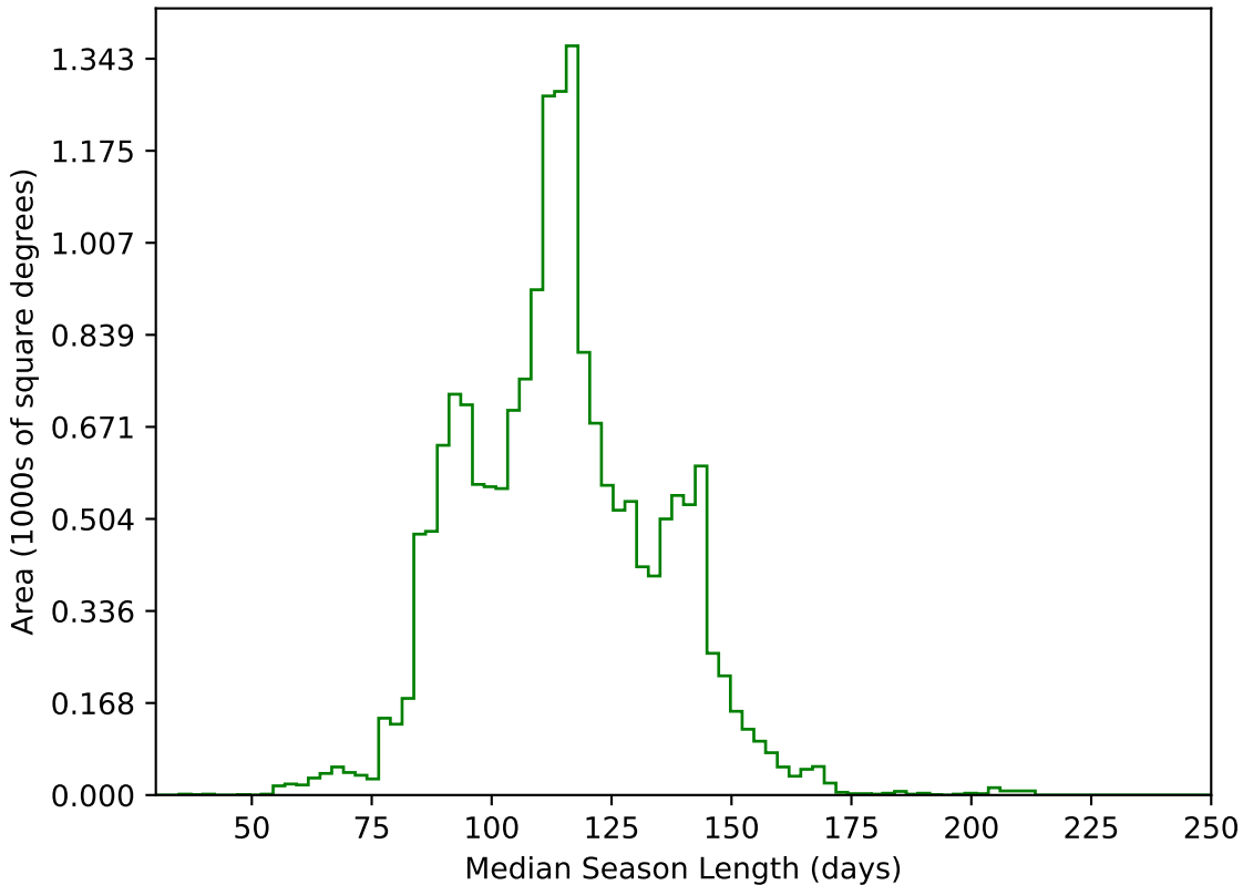
noroll_mjdp365_v3.4_10yrs WFD g band: Median Season Length
