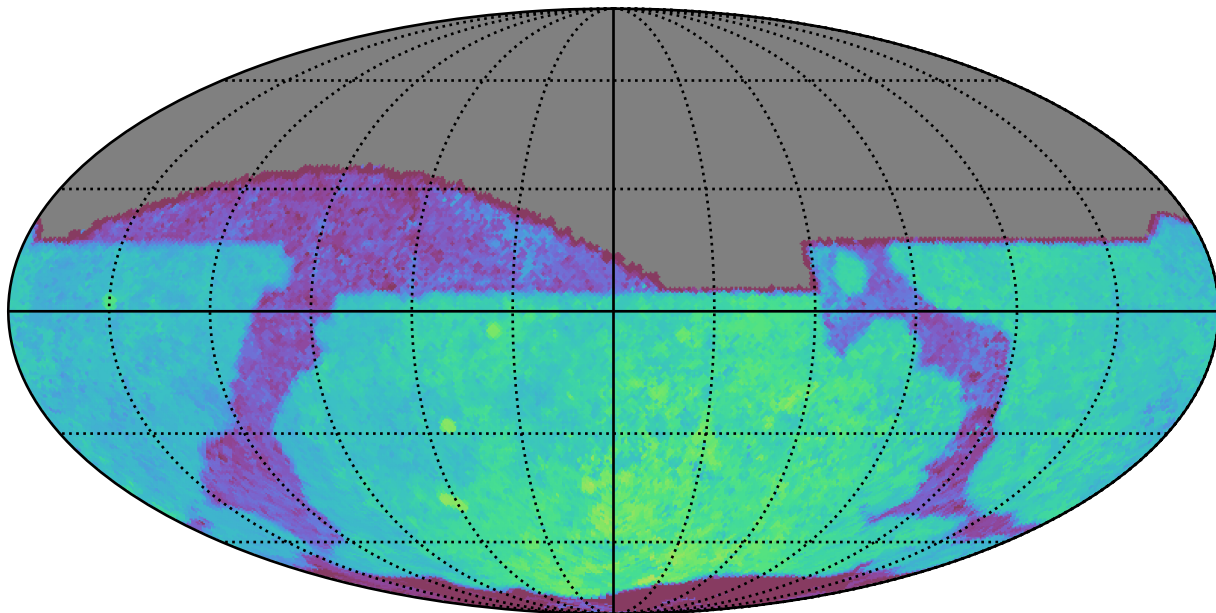
noroll_mjdp365_v3.4_10yrs All sky z band: Median Season Length
