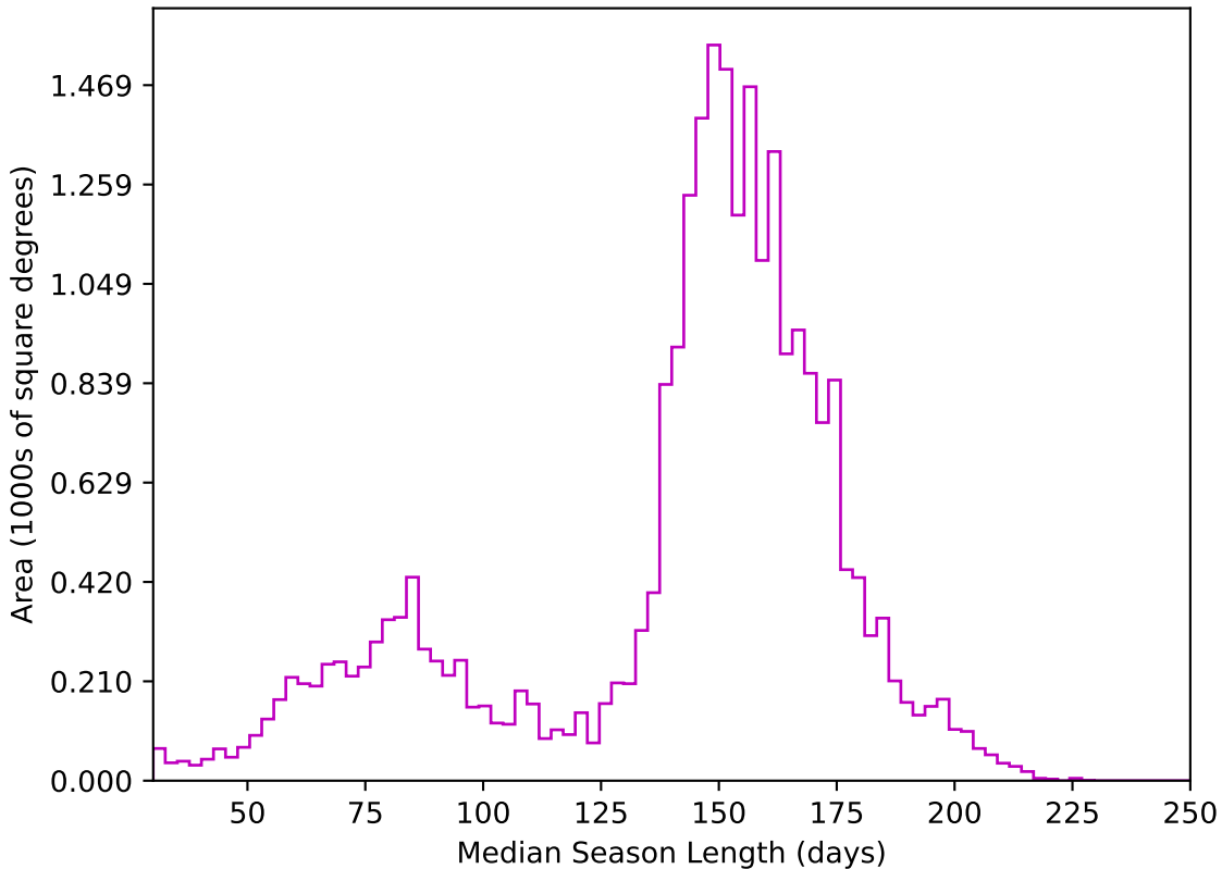
noroll_mjdp365_v3.4_10yrs All sky z band: Median Season Length
