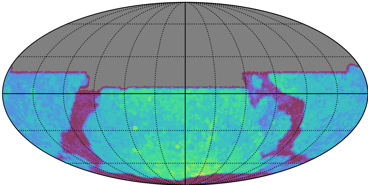
noroll_mjdp365_v3.4_10yrs All sky y band: Median Season Length
