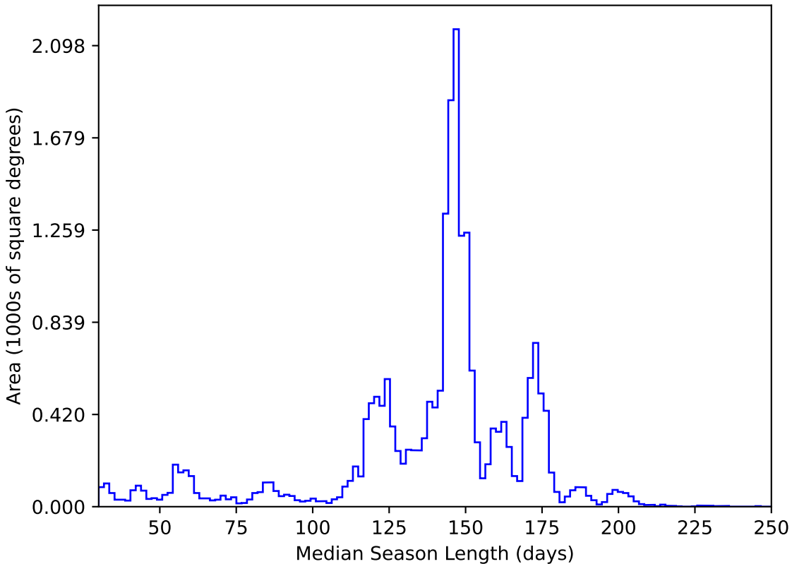
noroll_mjdp365_v3.4_10yrs All sky y band: Median Season Length
