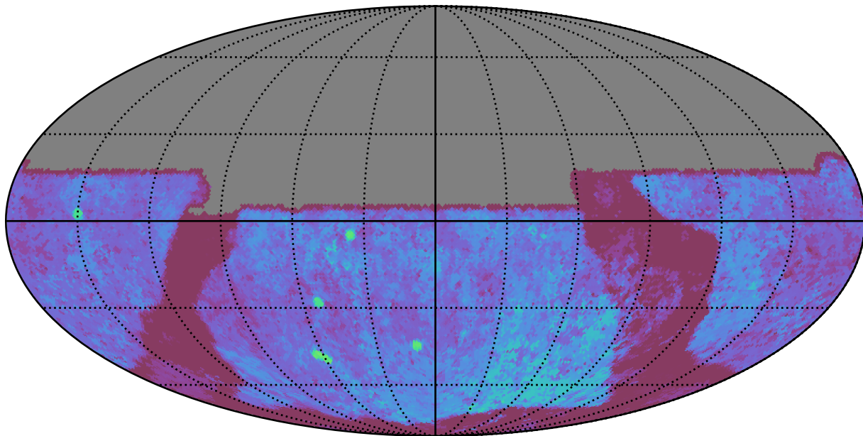
noroll_mjdp365_v3.4_10yrs All sky u band: Median Season Length
