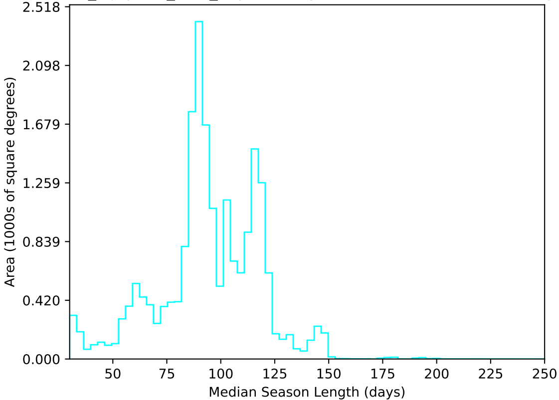
noroll_mjdp365_v3.4_10yrs All sky u band: Median Season Length
