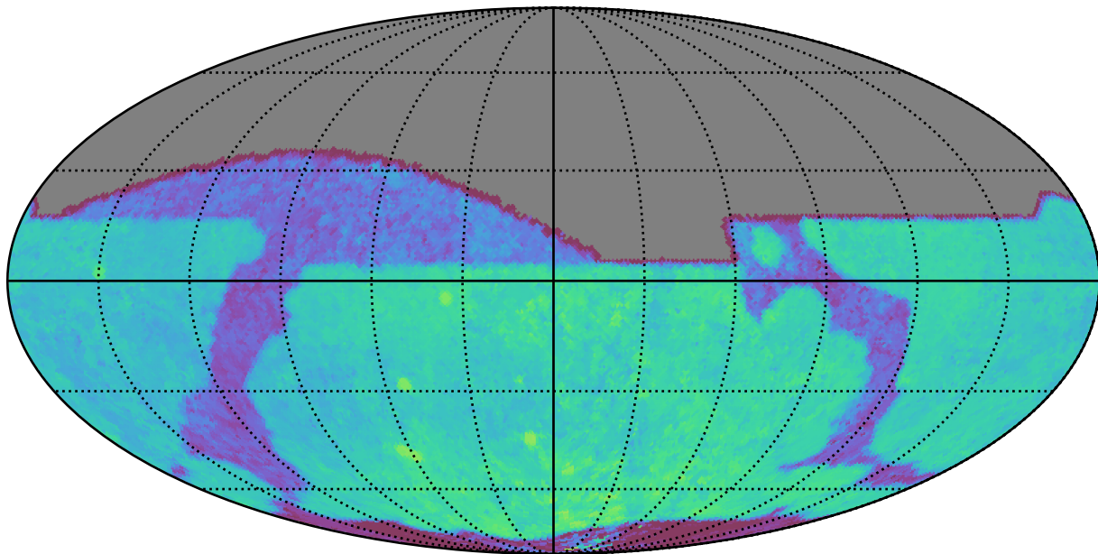
noroll_mjdp365_v3.4_10yrs All sky i band: Median Season Length
