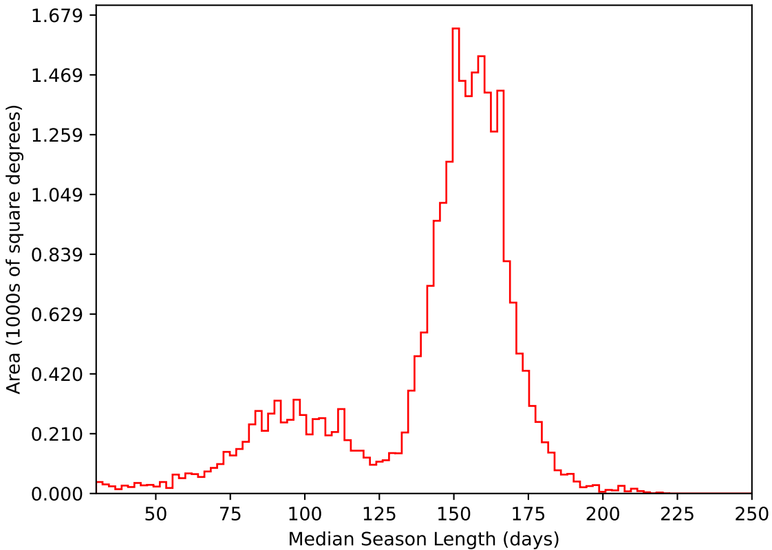
noroll_mjdp365_v3.4_10yrs All sky i band: Median Season Length
