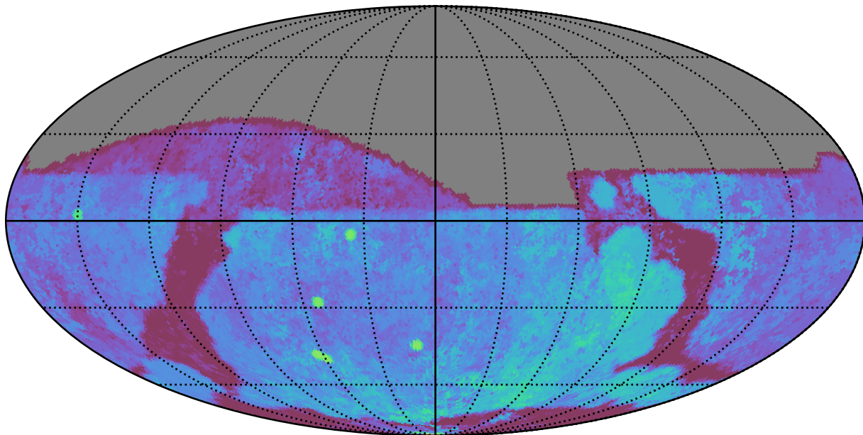
noroll_mjdp365_v3.4_10yrs All sky g band: Median Season Length
