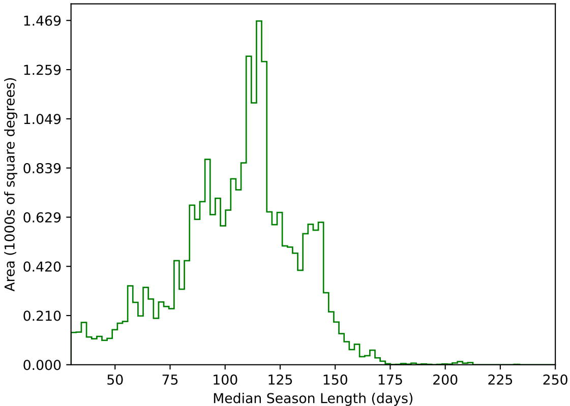
noroll_mjdp365_v3.4_10yrs All sky g band: Median Season Length
