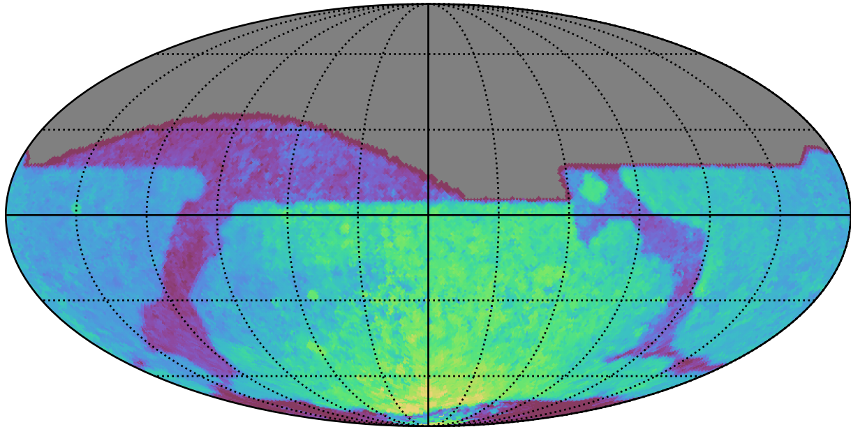
noroll_mjdp365_v3.4_10yrs All sky all bands: Median Season Length
