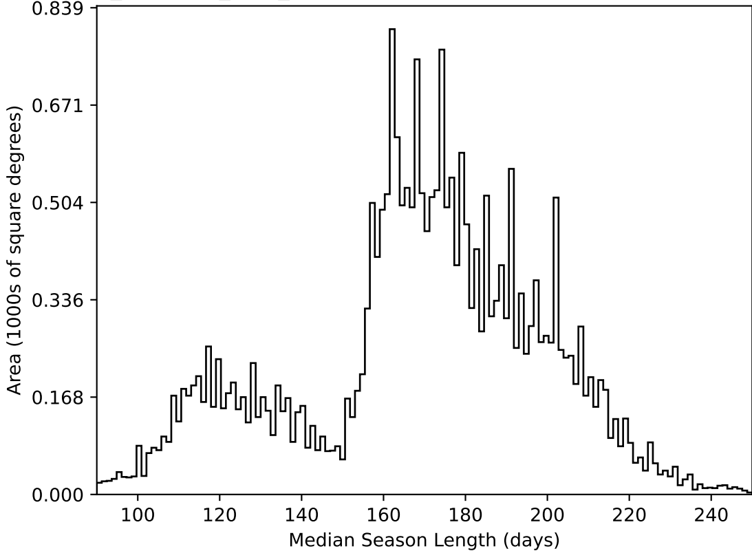
noroll_mjdp365_v3.4_10yrs All sky all bands: Median Season Length
