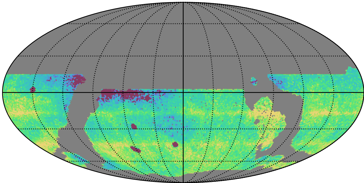
noroll_mjdp365_v3.4_10yrs WFD: Median Intra-Night Gap
