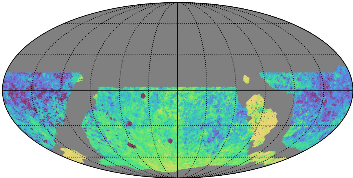
noroll_mjdp365_v3.4_10yrs WFD y band: Median Inter-Night Gap
