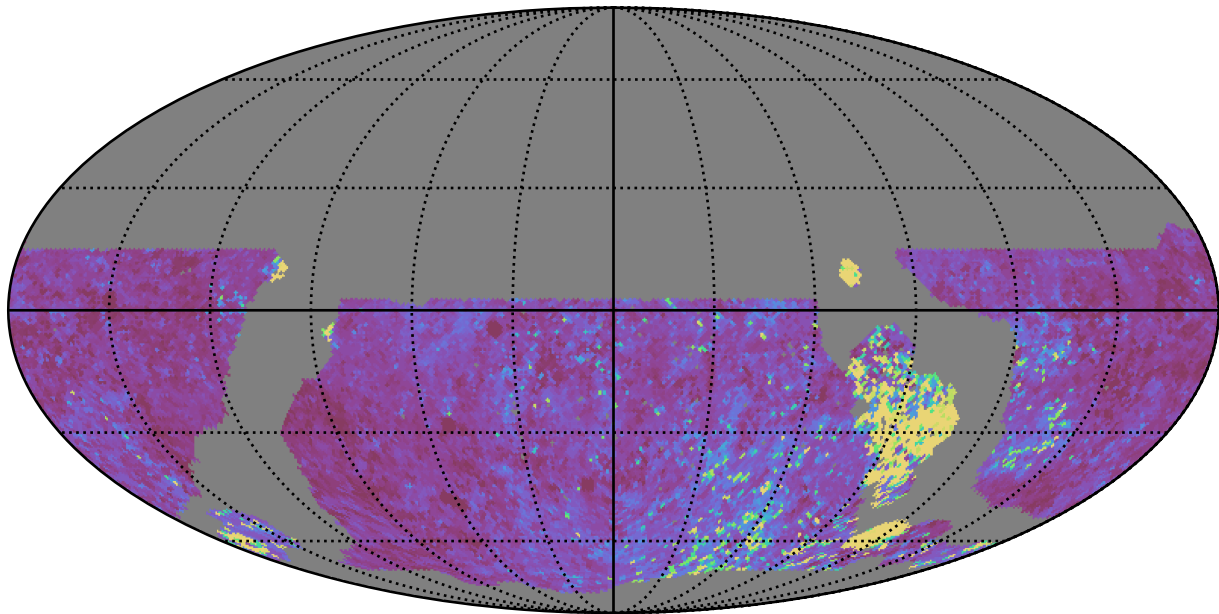
noroll_mjdp365_v3.4_10yrs WFD u band: Median Inter-Night Gap
