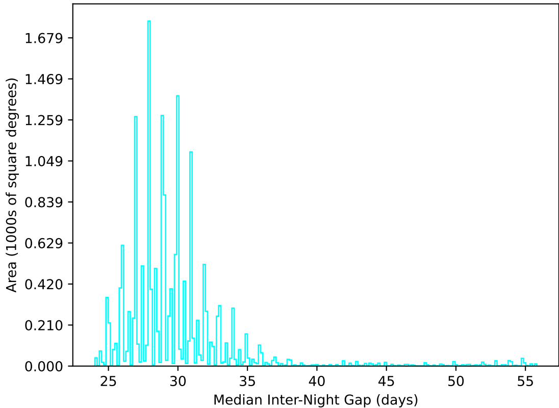
noroll_mjdp365_v3.4_10yrs WFD u band: Median Inter-Night Gap
