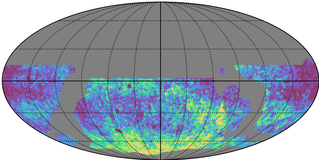
noroll_mjdp365_v3.4_10yrs WFD r band: Median Inter-Night Gap
