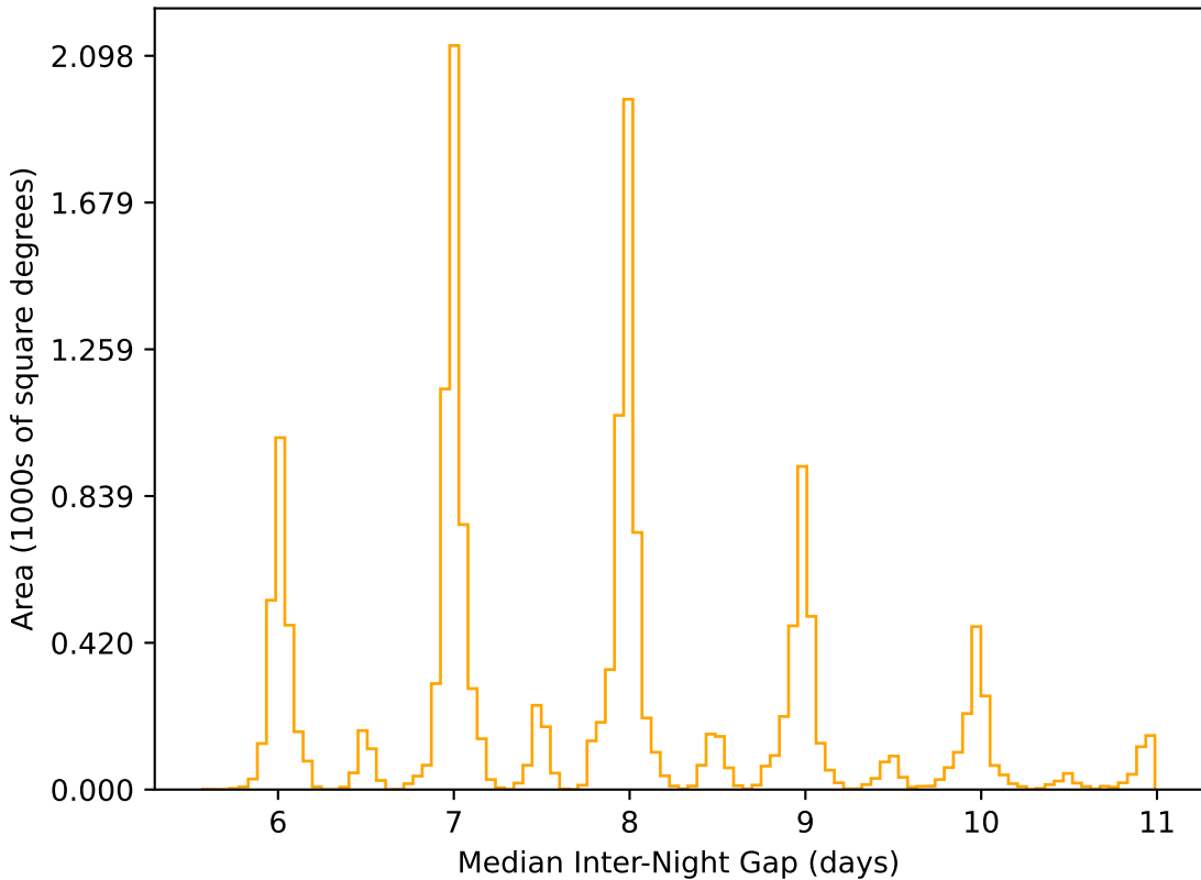
noroll_mjdp365_v3.4_10yrs WFD r band: Median Inter-Night Gap
