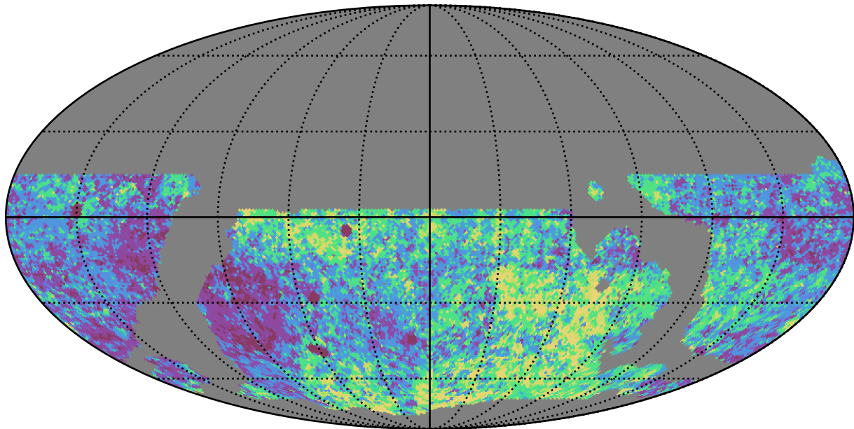
noroll_mjdp365_v3.4_10yrs WFD i band: Median Inter-Night Gap
