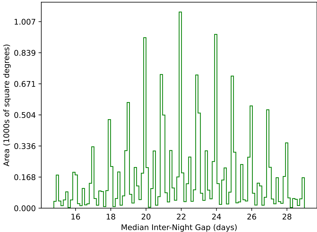
noroll_mjdp365_v3.4_10yrs WFD g band: Median Inter-Night Gap
