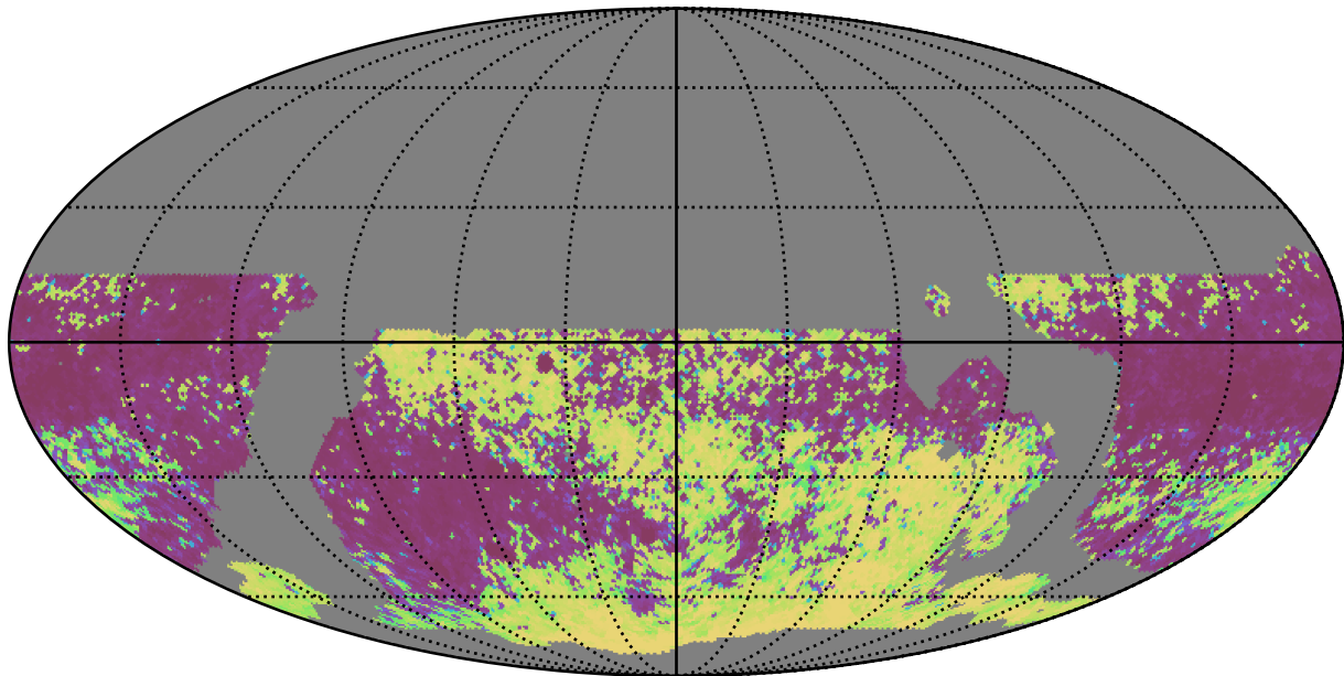
noroll_mjdp365_v3.4_10yrs WFD all bands: Median Inter-Night Gap
