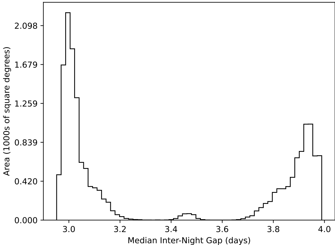
noroll_mjdp365_v3.4_10yrs WFD all bands: Median Inter-Night Gap
