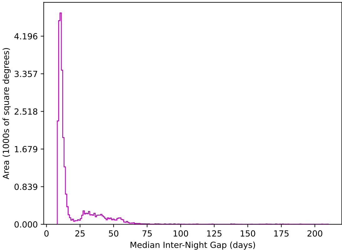
noroll_mjdp365_v3.4_10yrs All sky z band: Median Inter-Night Gap
