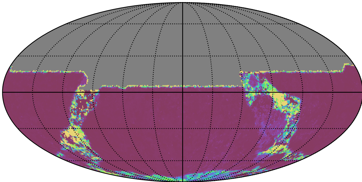
noroll_mjdp365_v3.4_10yrs All sky u band: Median Inter-Night Gap
