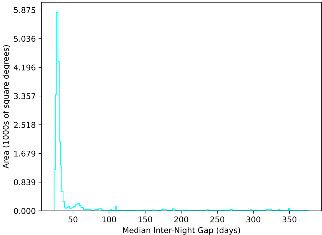
noroll_mjdp365_v3.4_10yrs All sky u band: Median Inter-Night Gap
