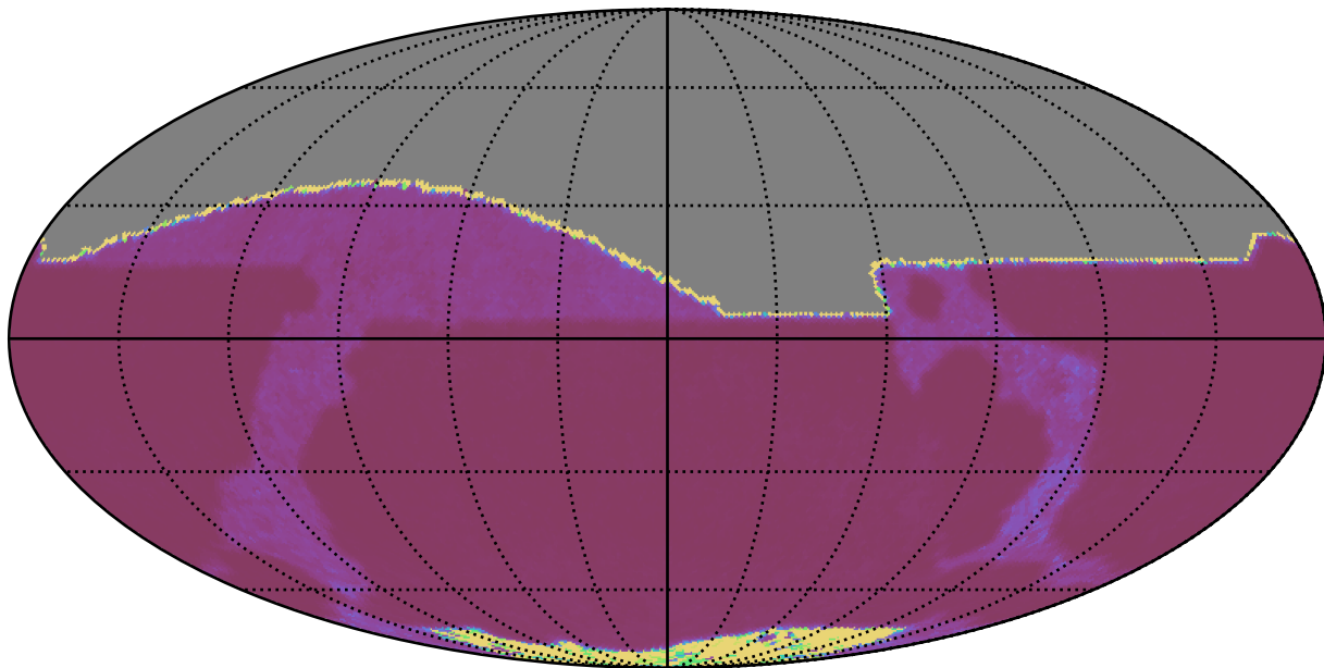
noroll_mjdp365_v3.4_10yrs All sky r band: Median Inter-Night Gap
