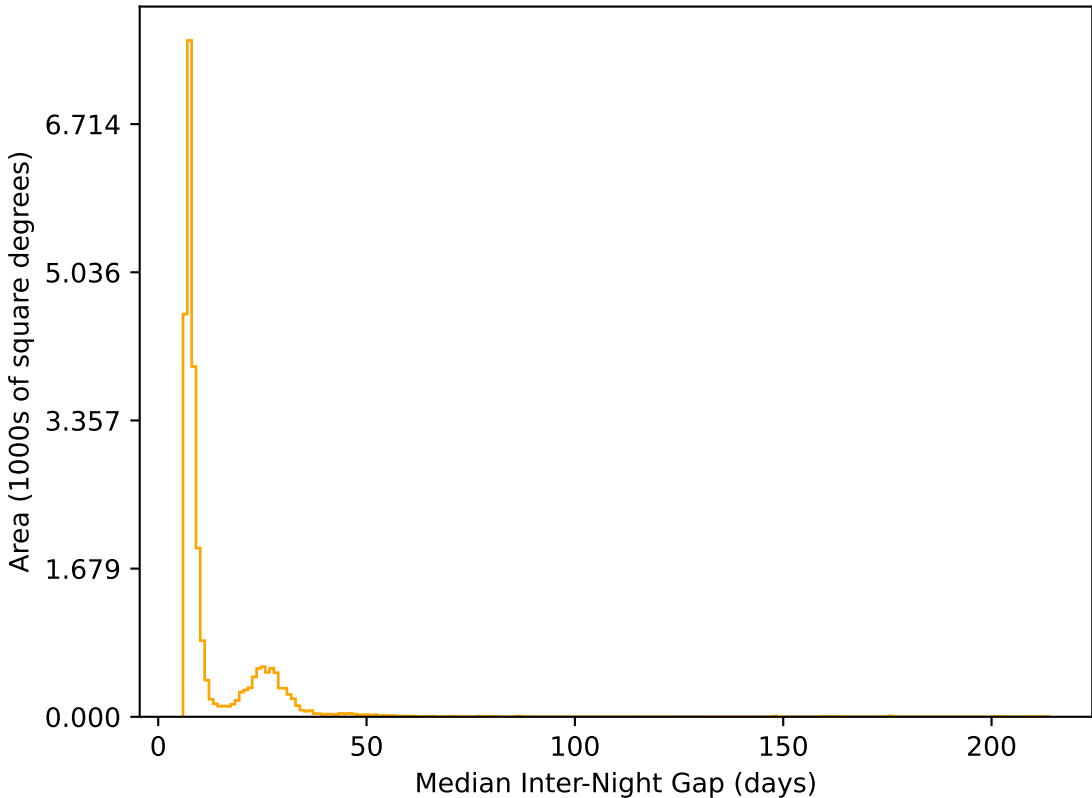
noroll_mjdp365_v3.4_10yrs All sky r band: Median Inter-Night Gap
