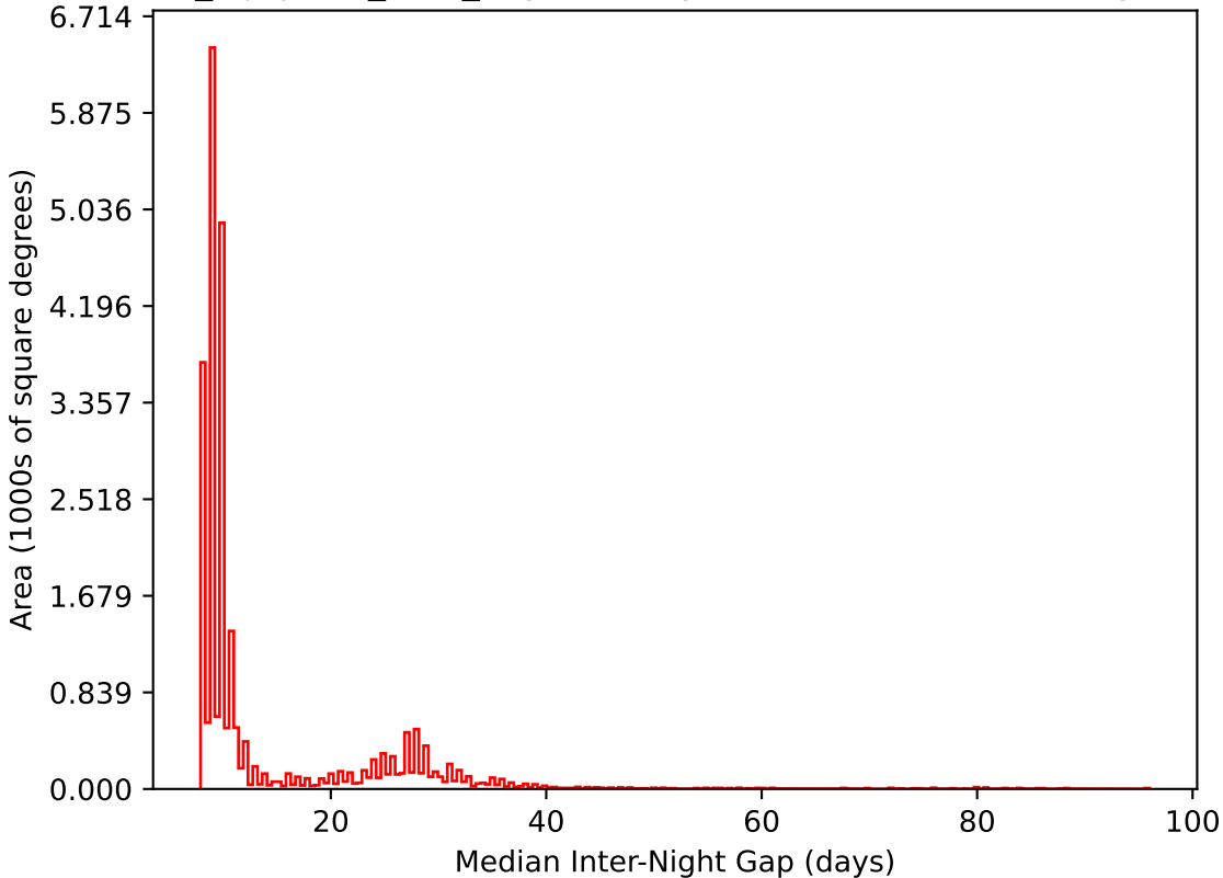
noroll_mjdp365_v3.4_10yrs All sky i band: Median Inter-Night Gap
