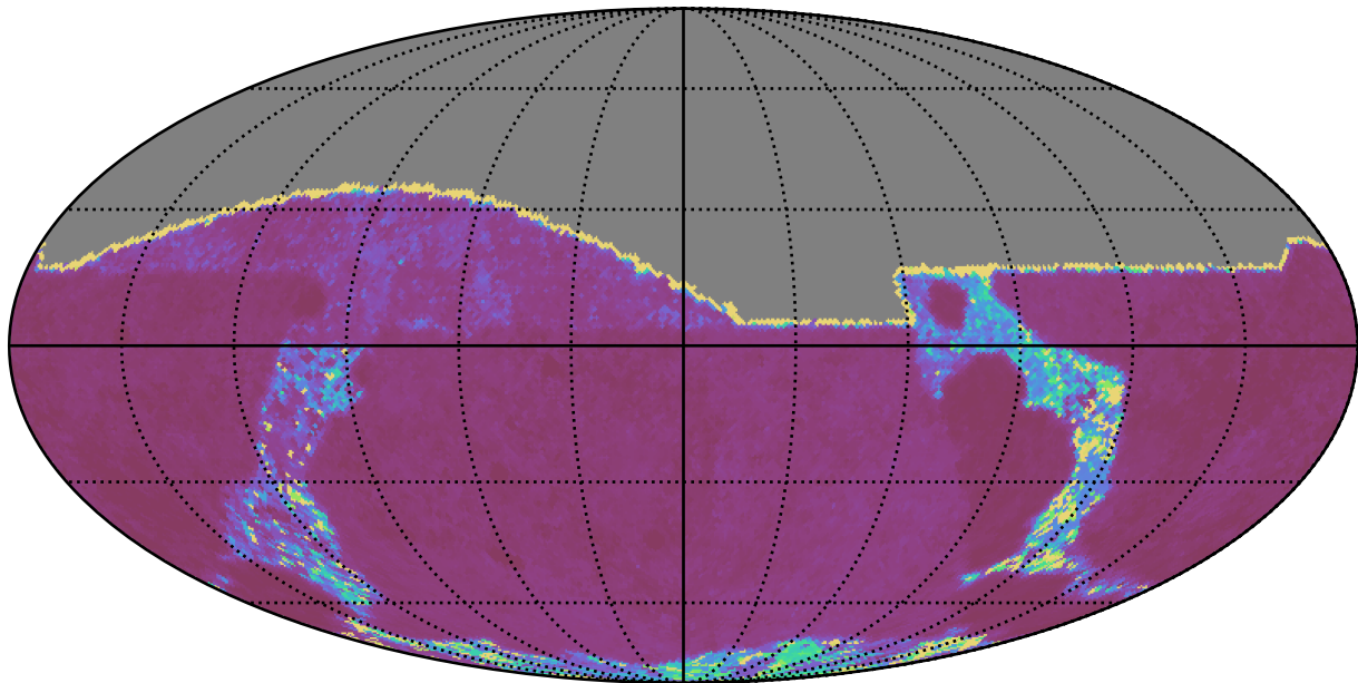
noroll_mjdp365_v3.4_10yrs All sky g band: Median Inter-Night Gap
