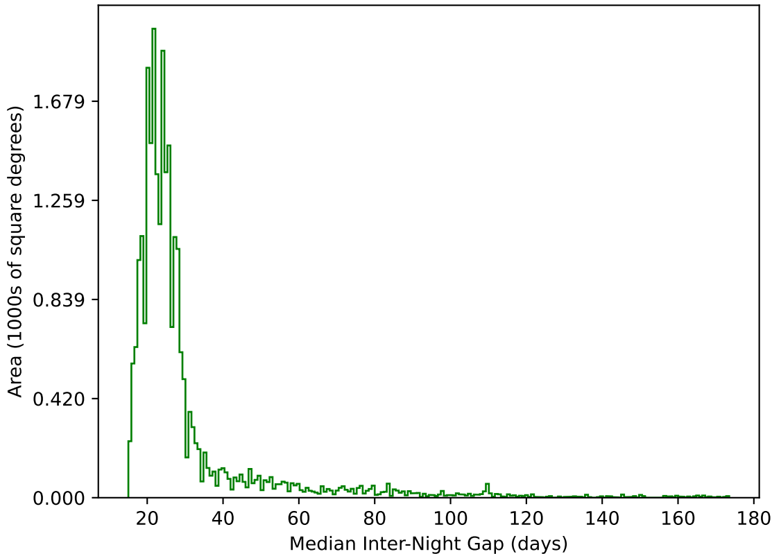
noroll_mjdp365_v3.4_10yrs All sky g band: Median Inter-Night Gap
