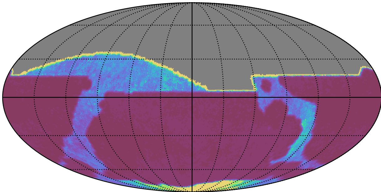
noroll_mjdp365_v3.4_10yrs All sky all bands: Median Inter-Night Gap
