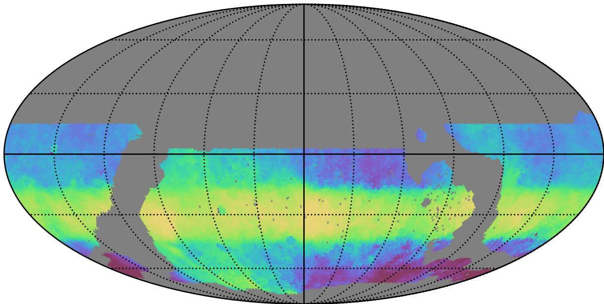
noroll_mjdp365_v3.4_10yrs WFD z band: Median HA
