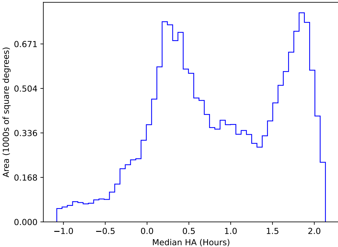
noroll_mjdp365_v3.4_10yrs WFD z band: Median HA
