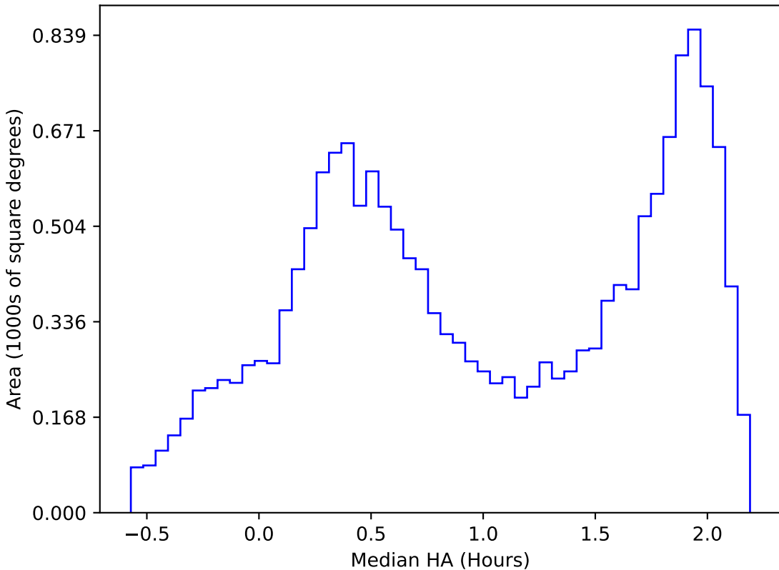
noroll_mjdp365_v3.4_10yrs WFD y band: Median HA
