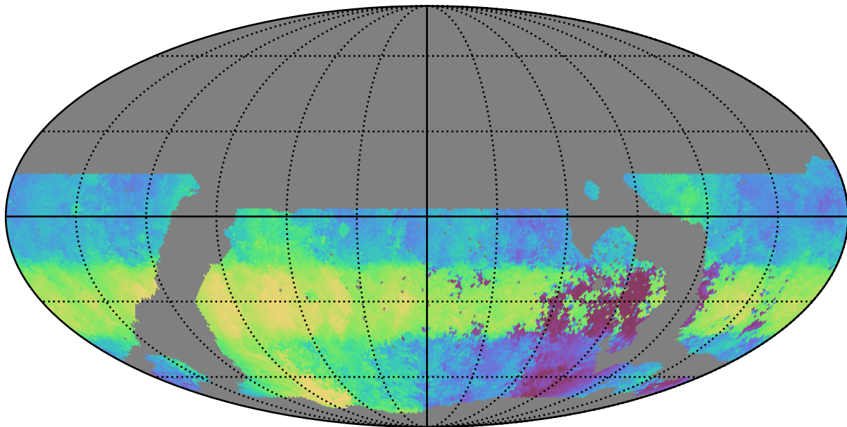
noroll_mjdp365_v3.4_10yrs WFD u band: Median HA
