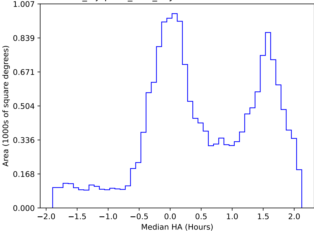
noroll_mjdp365_v3.4_10yrs WFD u band: Median HA
