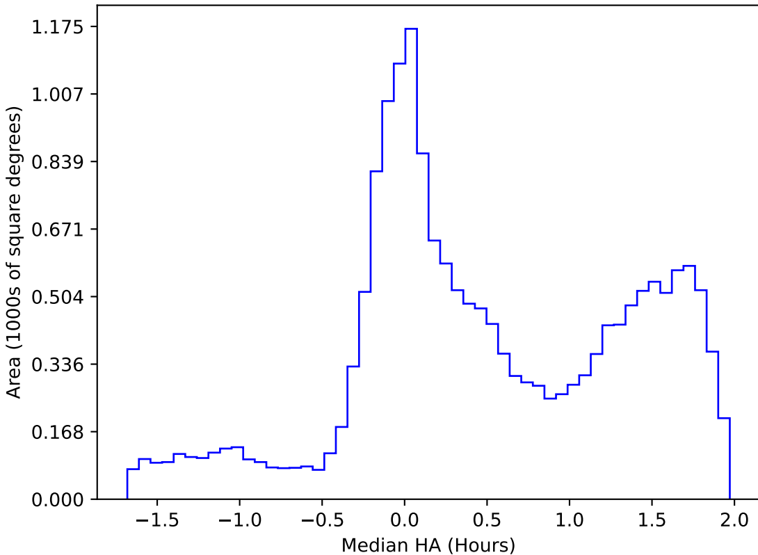
noroll_mjdp365_v3.4_10yrs WFD r band: Median HA
