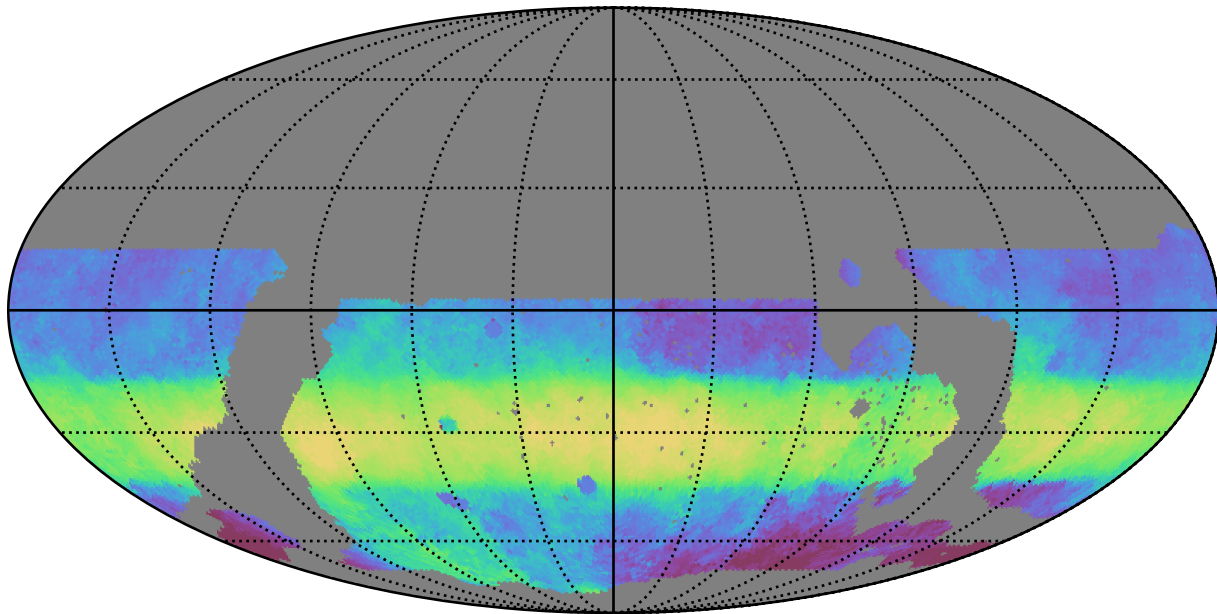
noroll_mjdp365_v3.4_10yrs WFD i band: Median HA
