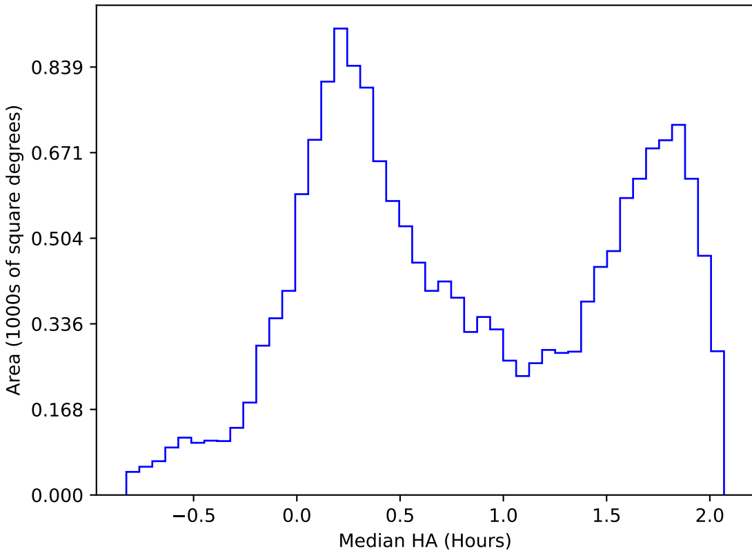
noroll_mjdp365_v3.4_10yrs WFD i band: Median HA
