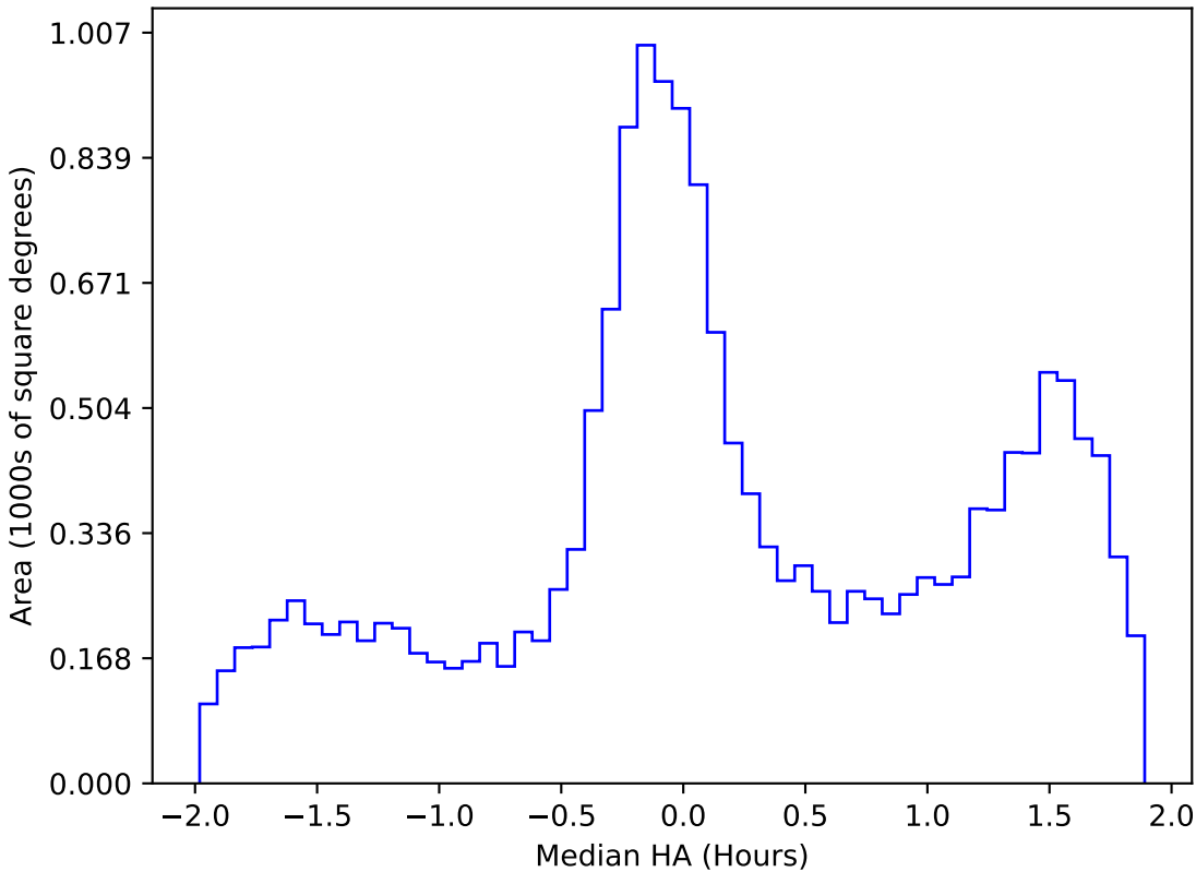
noroll_mjdp365_v3.4_10yrs WFD g band: Median HA
