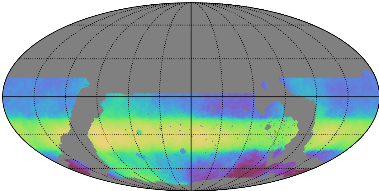
noroll_mjdp365_v3.4_10yrs WFD all bands: Median HA
