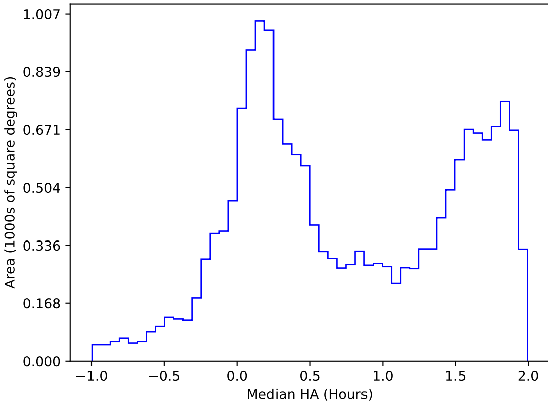
noroll_mjdp365_v3.4_10yrs WFD all bands: Median HA
