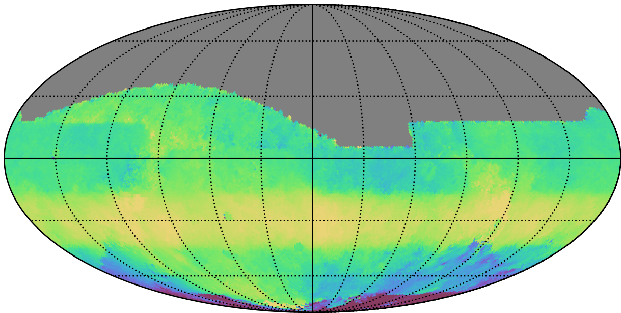
noroll_mjdp365_v3.4_10yrs All sky z band: Median HA
