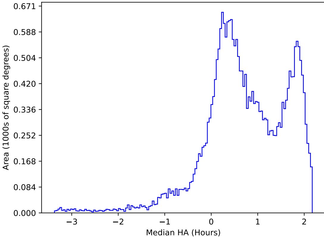
noroll_mjdp365_v3.4_10yrs All sky z band: Median HA
