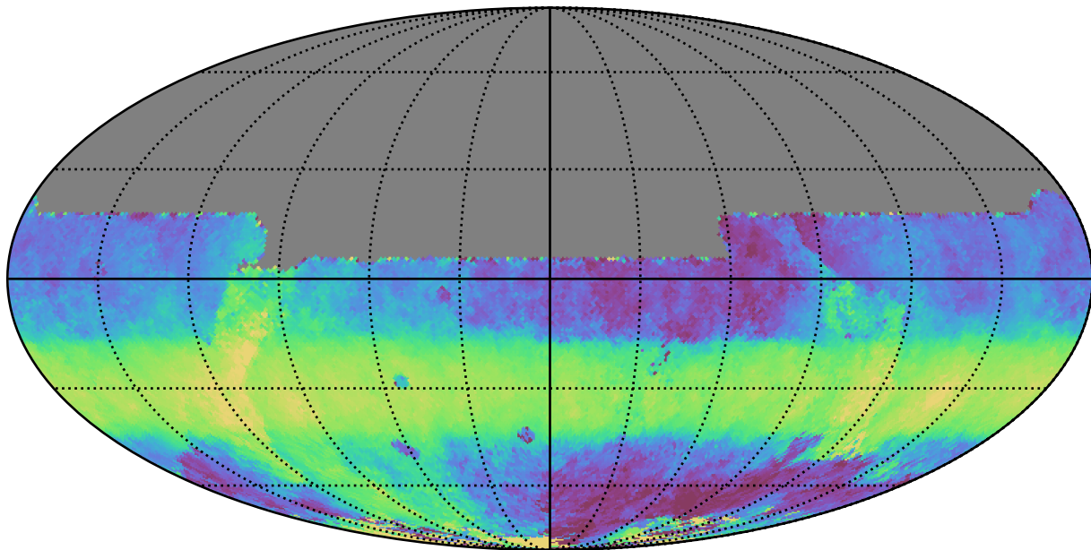
noroll_mjdp365_v3.4_10yrs All sky y band: Median HA
